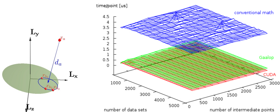
Fig. 2. Comparison of performance: The Gaalop code is up to fourteen times faster than the conventional math. The CUDA implementation gives a further performance improvement.
